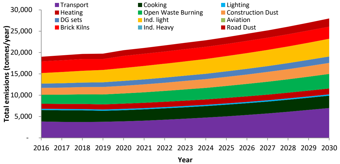
Figure 6: PM2.5 emissions (BAU)
