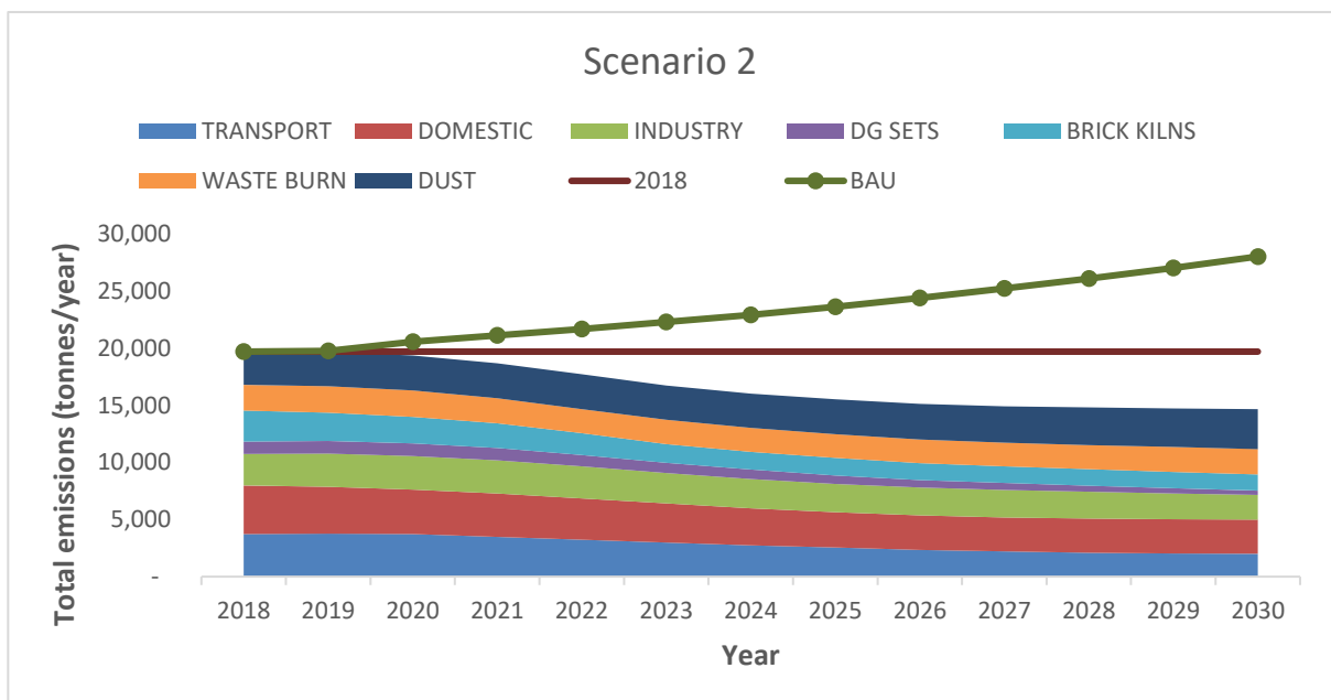
Figure 13: PM2.5 emissions scenario 2
