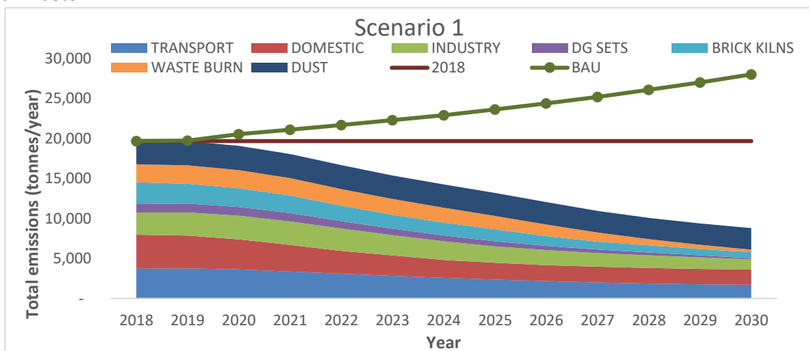
Figure 12: PM2.5 emissions scenario 1
