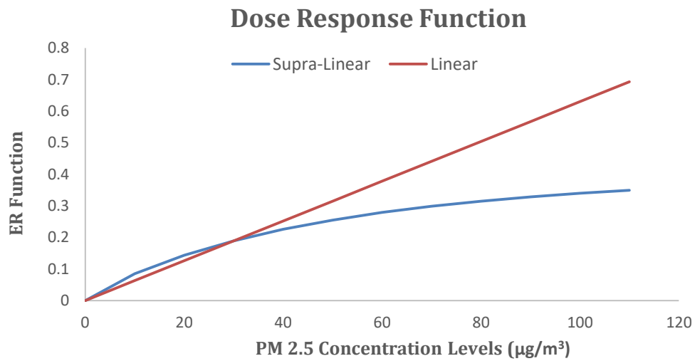
Figure 11: Supra-linear and linear form of ER function
