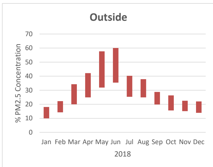
Figure 8: Sectoral share of PM2.5 concentration levels (%) (2018)
