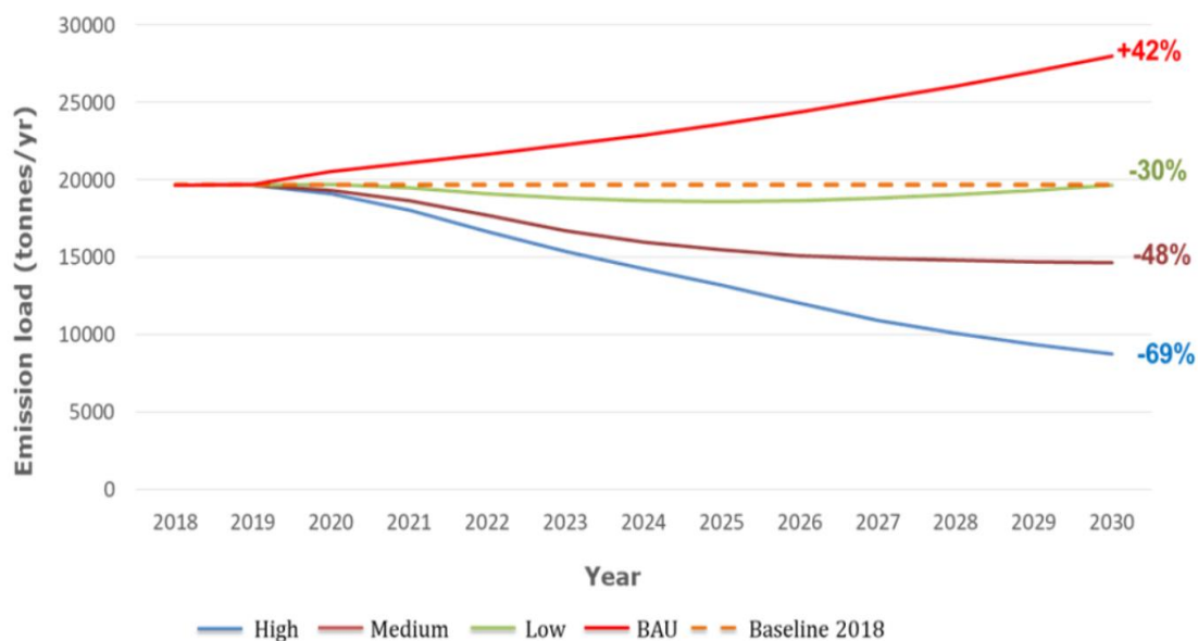
Figure 15: Pollution reduction potential scenarios
