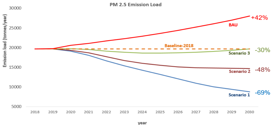
Figure 2: Scenarios: emission-reduction potential
