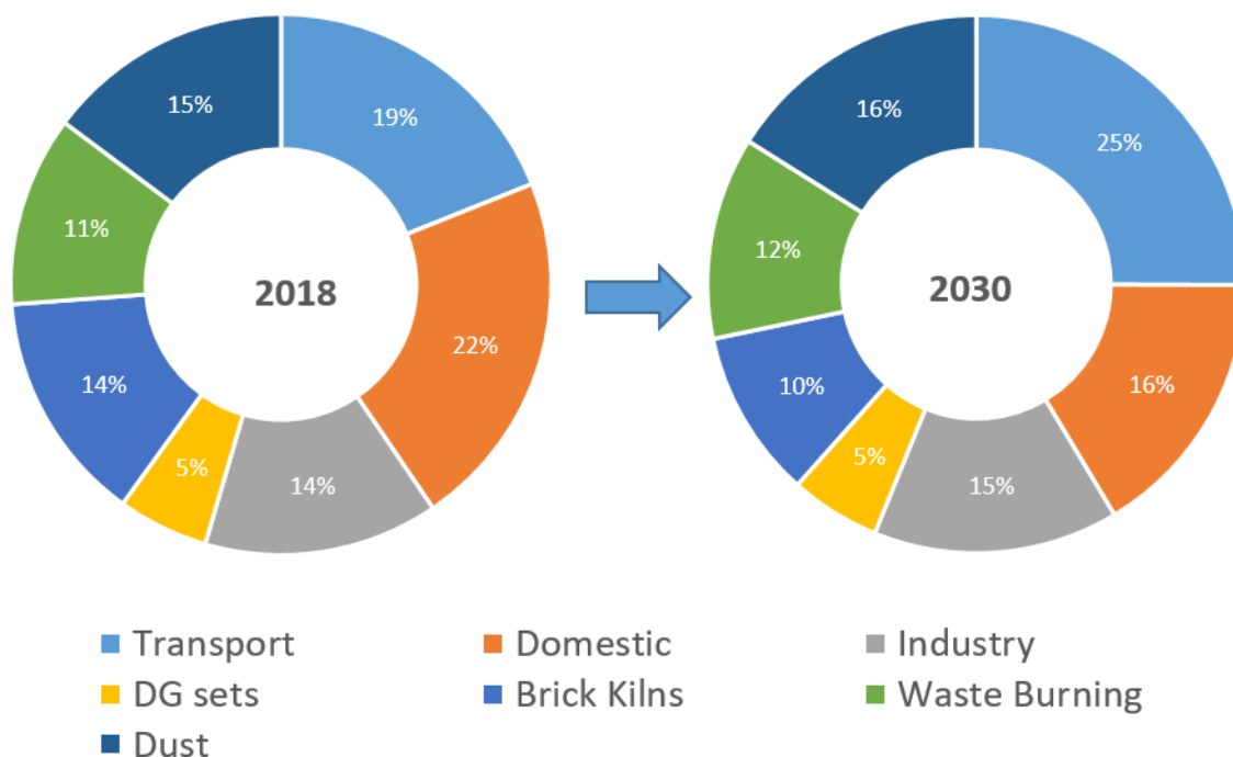
Figure 1: Patna emission load (BAU)
