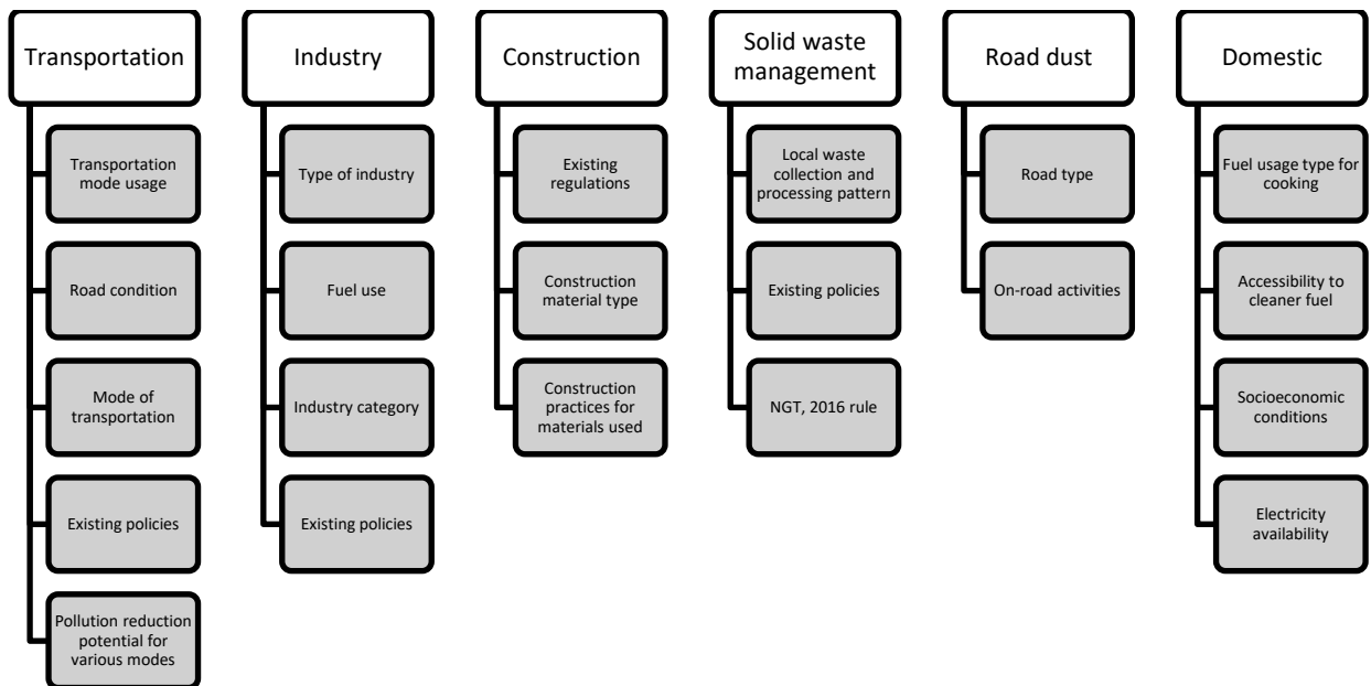
Figure 10: Determinants for source-specific CMs
