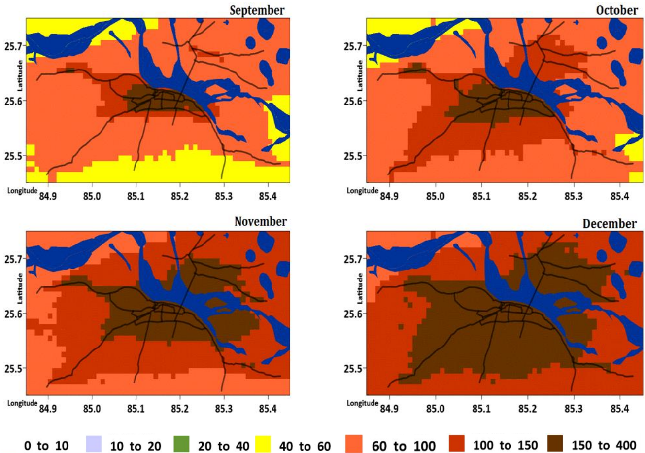
Figure 7: PM2.5 concentration levels ( \mu\text{g}/\text{m}^3 ) (BAU-2018)
