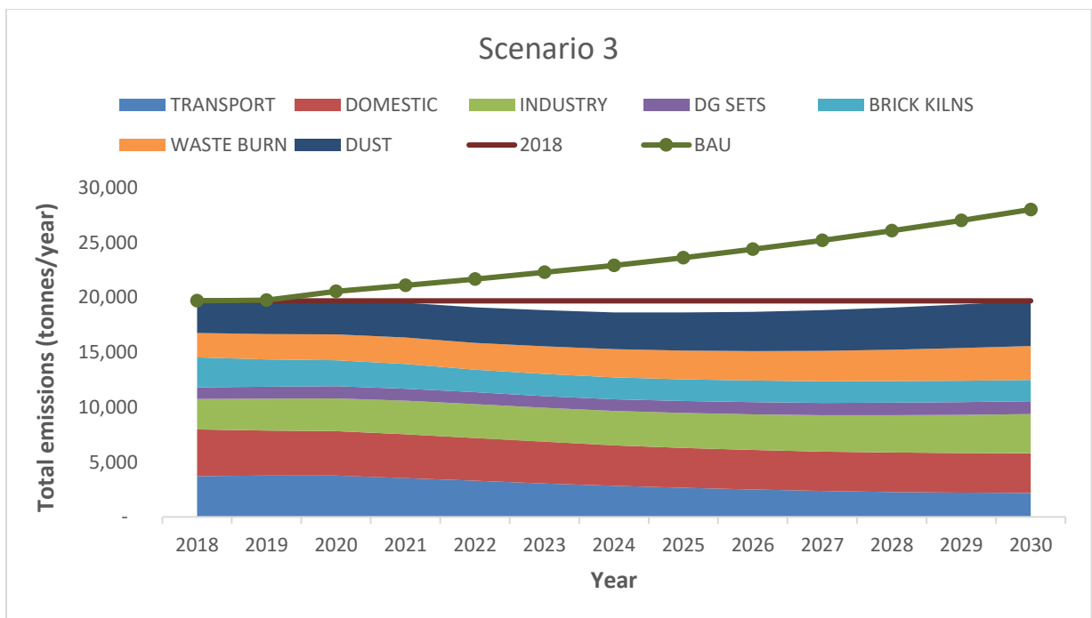
Figure 14: PM2.5 emissions scenario 3
