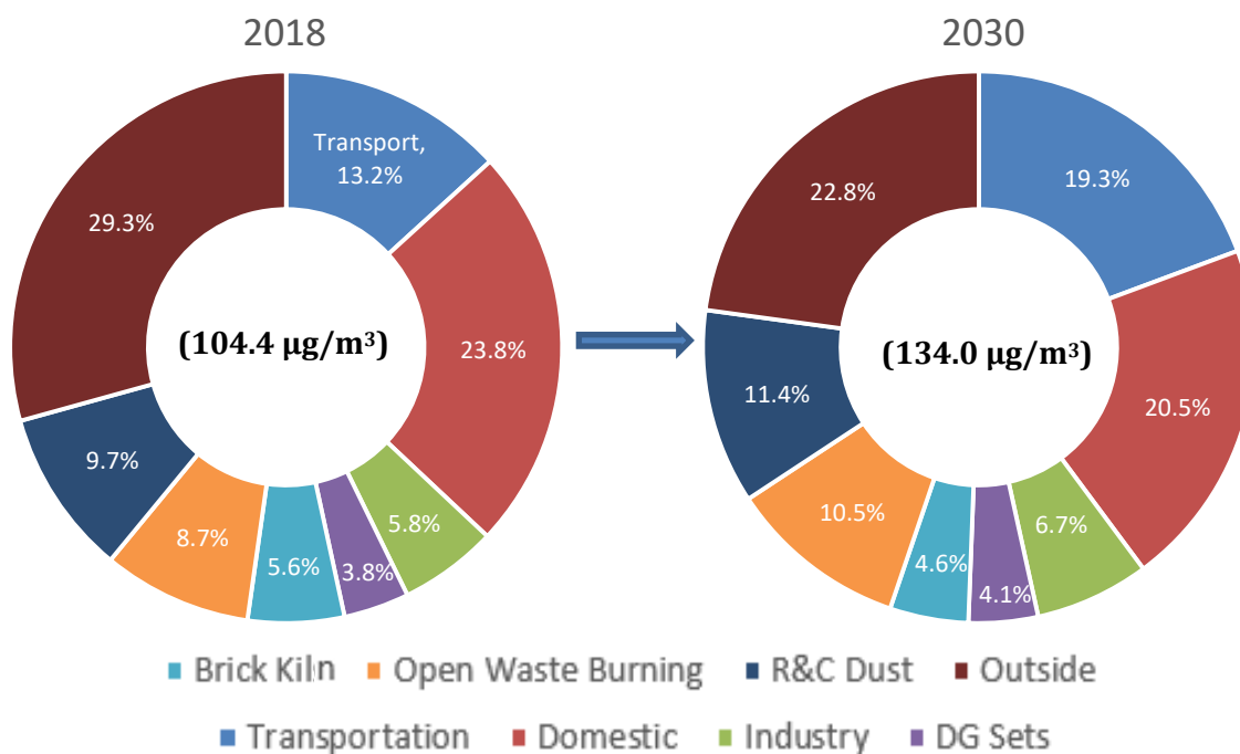
Figure 9: PM2.5 concentration levels (BAU) 2018 vs 2030
