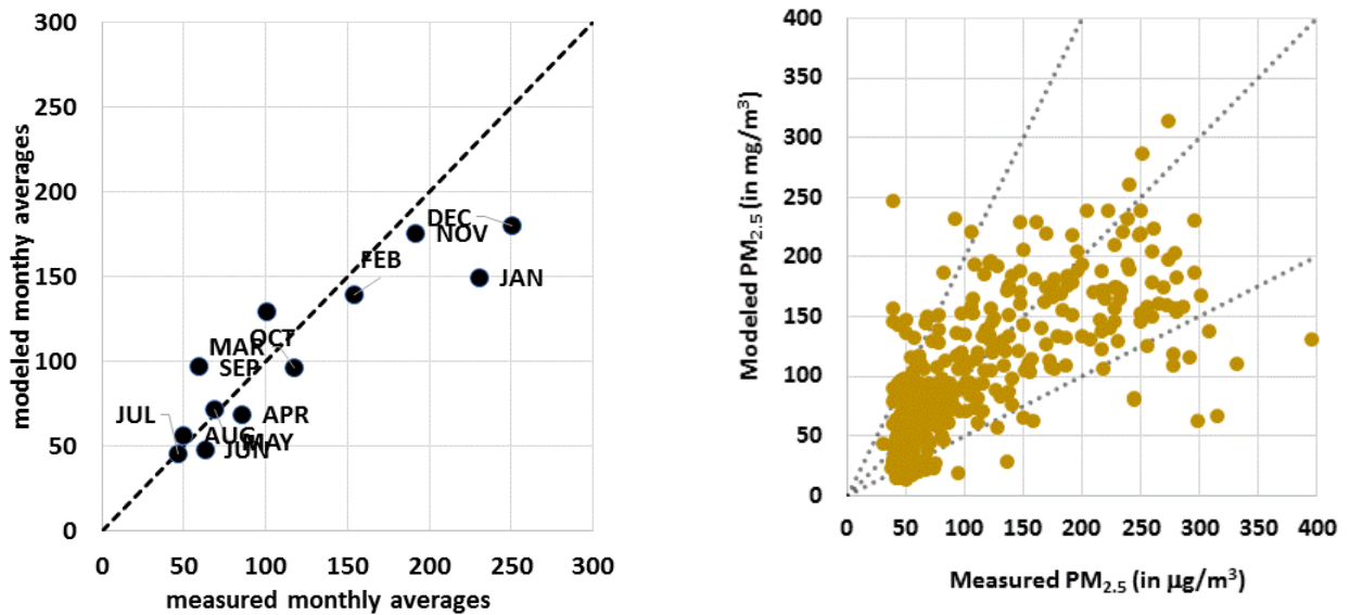
Figure 5: Modelled vs measured PM2.5
